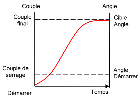
FIGURE 50 - Mode angle
